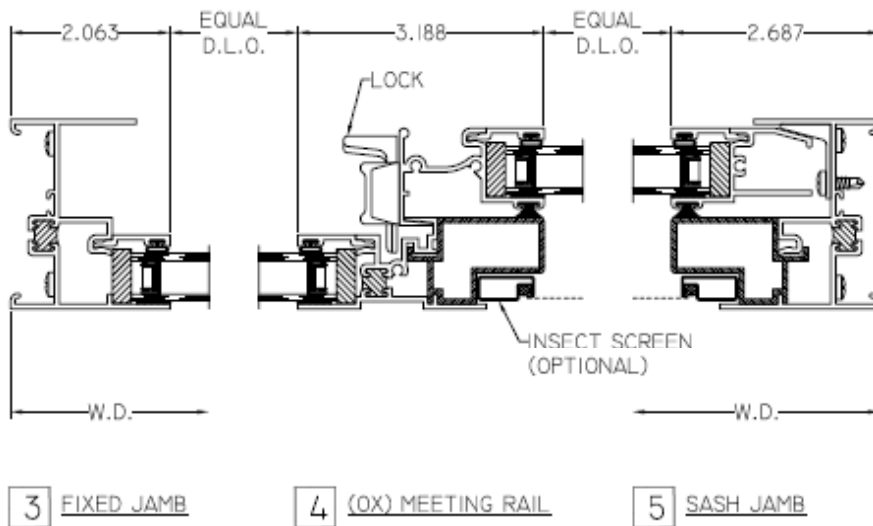
HALF SCALE DETAILS
